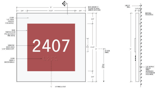
ROOM NUMBER PART# 4P19-1000-R
